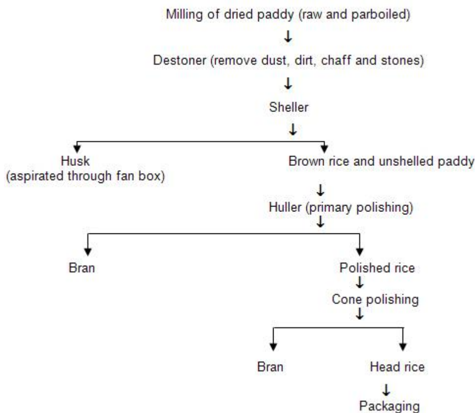
Fig. 2 Process flow diagram of paddy milling
