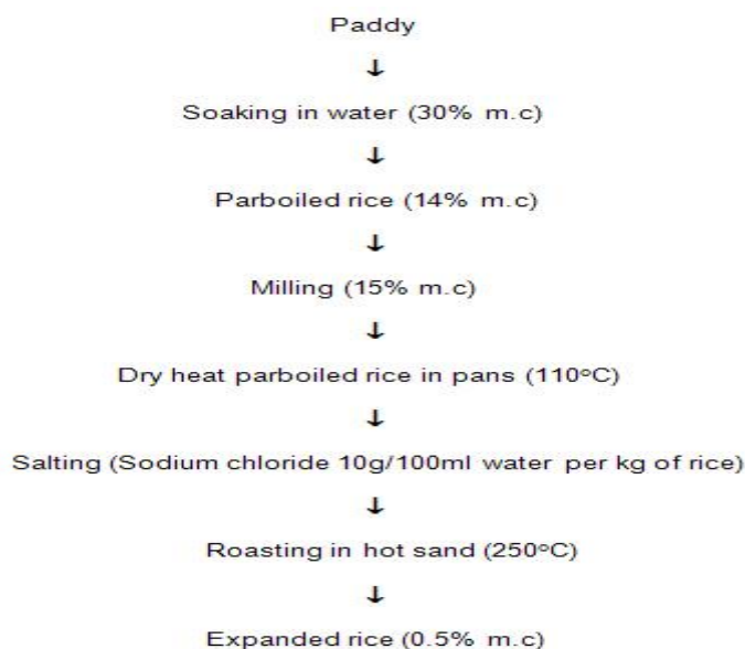
Fig. 11 Processing steps of Parched rice
