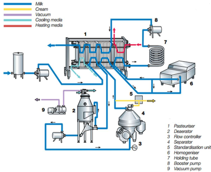
Fig: Typical Milk Pasteurizer Unit
