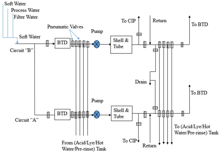
Fig: A two station CIP Circuit
